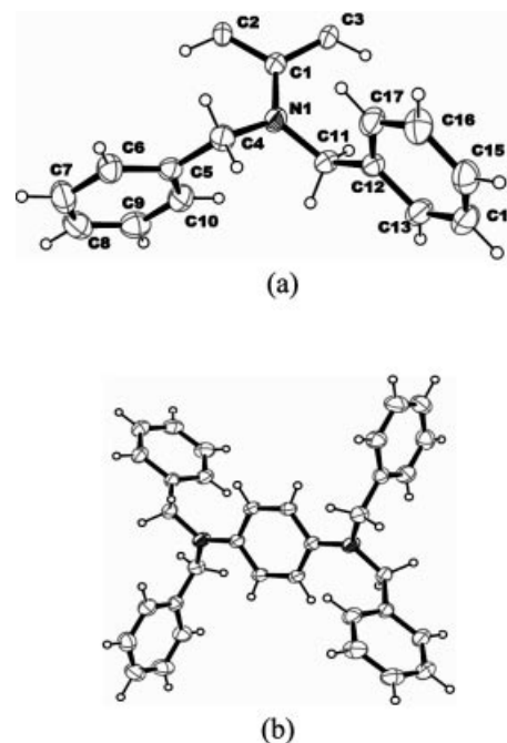
Figure 1. (a) ORTEP plot with the atom numbering of asymmetric unit 9a ; (b) ORTEP plot of 9a .
